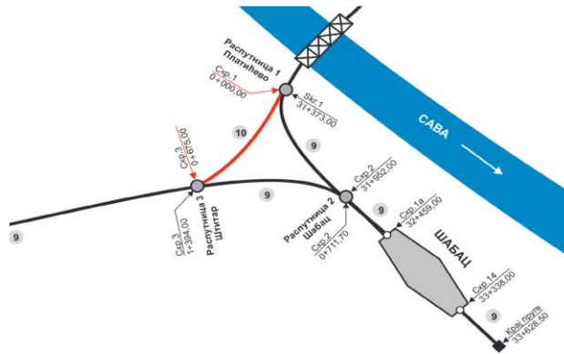
Figure 2. Track alignment at Šabac triangle and at the end of rail line
